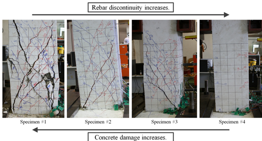
Fig. 19. Degree of deterioration for each specimen versus number of discontinuous reinforcing bars
