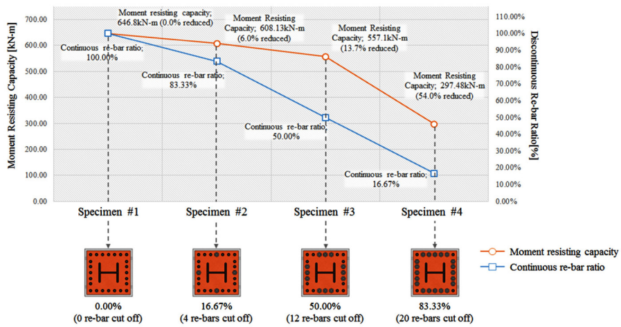
Fig. 18. Maximum moment resisting capacity versus number of continuous reinforcing bars
